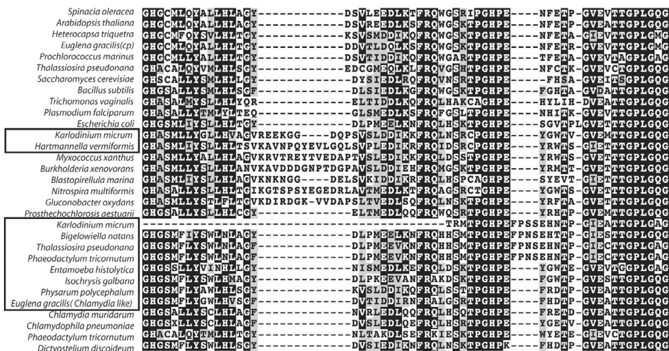
Figure 4 Transketolase alignment flanking a 4-amino acid insertion present in diatom, dinoflagellate and chlorarachnio-phyte TK-Ch genes. A nearby 11- to 15-amino acid insertion characterizes a mixed group of CFB bacteria and proteobacteria as well as the amoebozoan Hartmannella vermiformis and the dinoflagellate Karlodinium micrum . Eukaryotic TKs putatively derived from lateral transfer events are surrounded by black squares (TK-Ch being the lower box).
